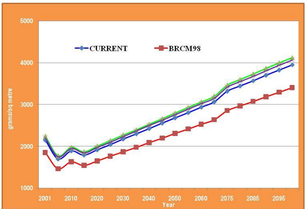
Figure 5.13: Projections of organic matter content (g/m 2 ) in soil at the Dankunku rangelands. “CURRENT” in this depiction of simulation results refers to the Reference/Baseline Climate Scenario. Green and Black lines that closely track the Baseline Scenario results are associated with the CCC199 and GDFL90 scenarios respectively.
