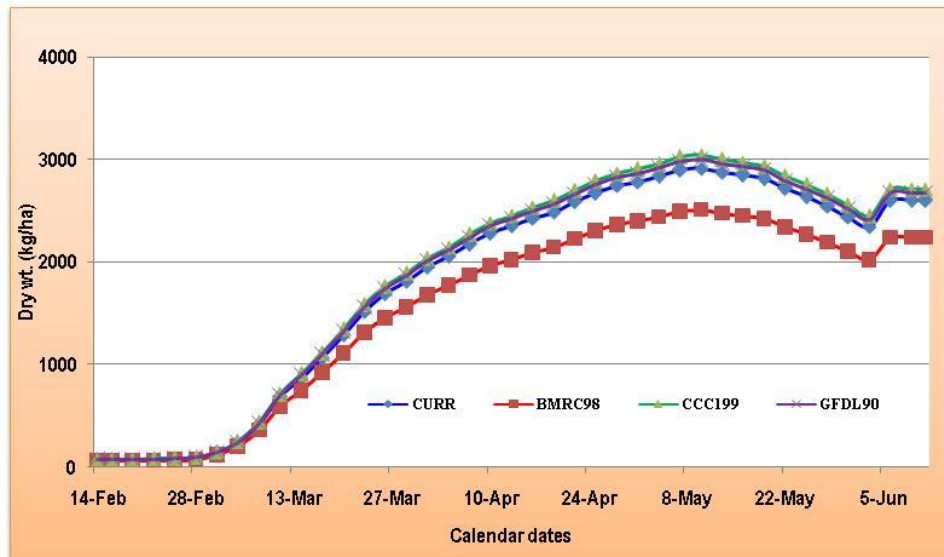
Figure 5.18: Simulated leaf dry weight (kg/ha) of irrigated rice at Kuntaur (The Gambia). Under the reference climate change scenario, simulated leaf dry weight at the end of the crop cycle lies between 2250 kg/ha (BMRC98) and 2700 kg/ha (CCC199). “CURR” in this depiction of simulation results refers to the Reference/Baseline Climate Scenario.
